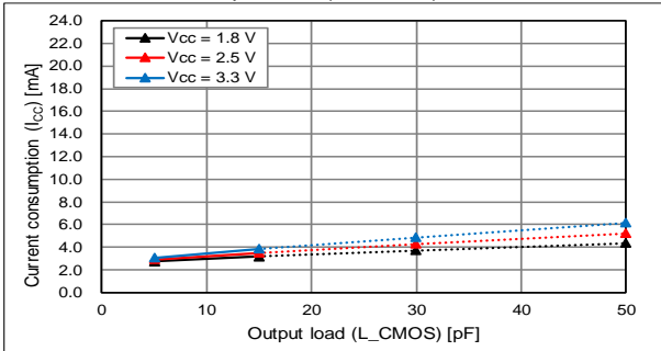
T use = +25 °C, Output load (L CMOS ) Characteristics
