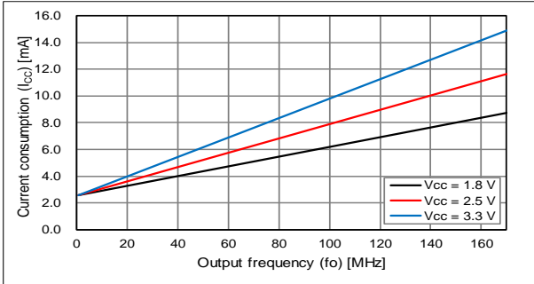
L CMOS = 15 pF, T use = +25 °C, Freq. Dependency
