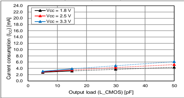
T use = +25 °C, Output load (L CMOS ) Characteristics
