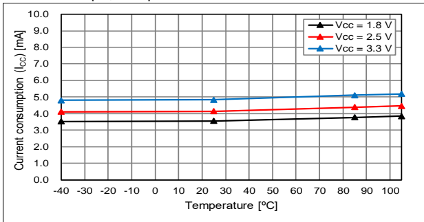
L CMOS = 5 pF, Temperature Characteristic
