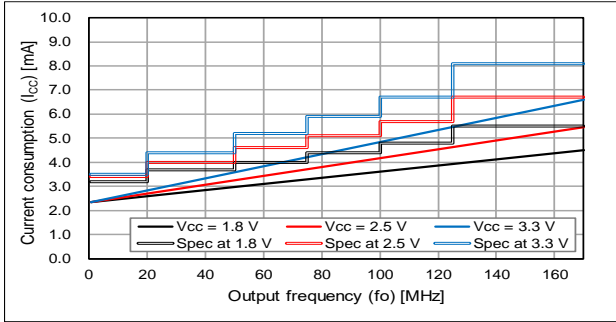
No load, T use = +25 °C, Freq. Dependency
