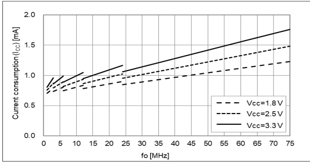
No load, T_{use} = +25\text{ }^{\circ}\text{C} , Freq. Dependency
