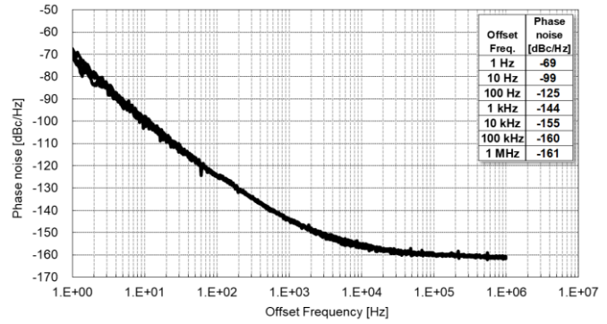
(4) fo = 19.2 MHz, T_use = +25 °C, n = 5 pcs
