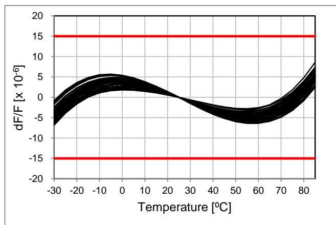
Frequency vs. Temperature characteristics (Frequency = 59.97MHz, n = 50)
