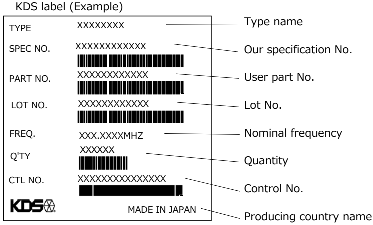
Pb-free label
