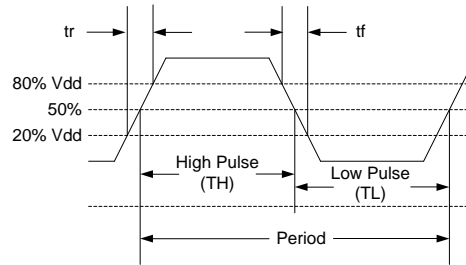
Figure 2. Waveform
