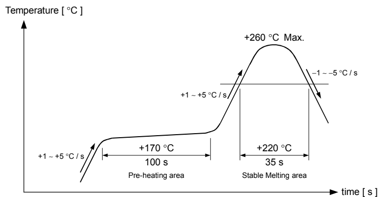
Fig. 1 : Reference profile for our evaluation of Soldering heat resistance.
