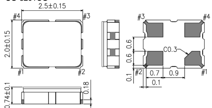
SG-8201CG
